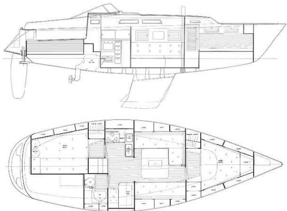
hallberg-rassy_34_drawing
