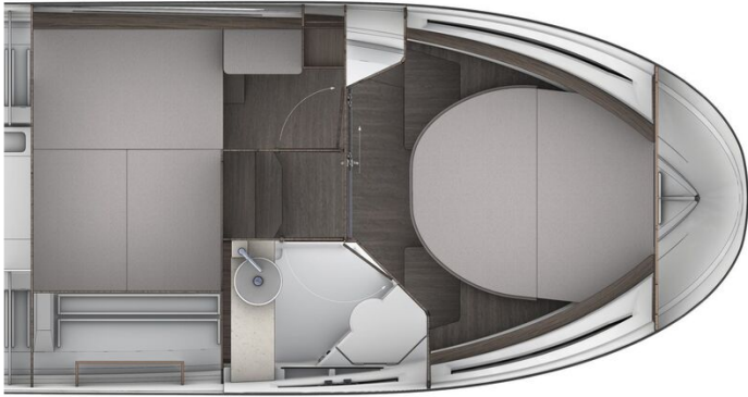
Jeanneau Merry Fisher 895 - diagram of cabins layout
