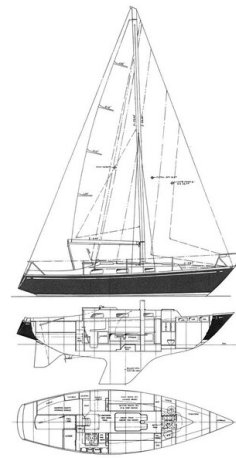
S & S 30 IVALU Layout
